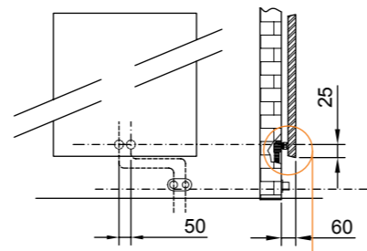
VALVOLA SATELLITE
